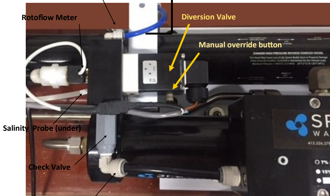
Product Diversion Valve Manifold
