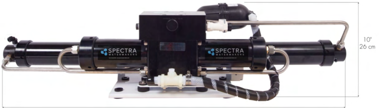
44" / 112 cm High Pressure Clark Pump and Membrane Depth 12" / 30.5 cm
