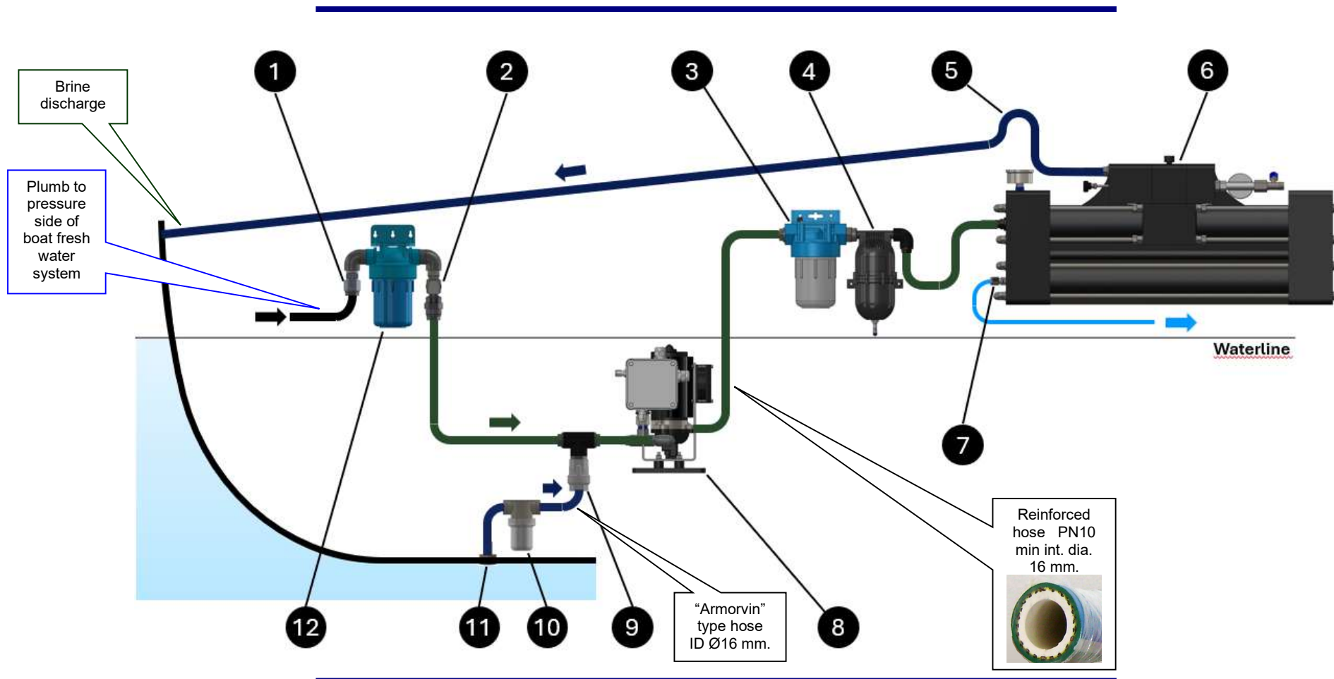
HYDRAULIC CONNECTION AND PIPES FIG. 4-7
