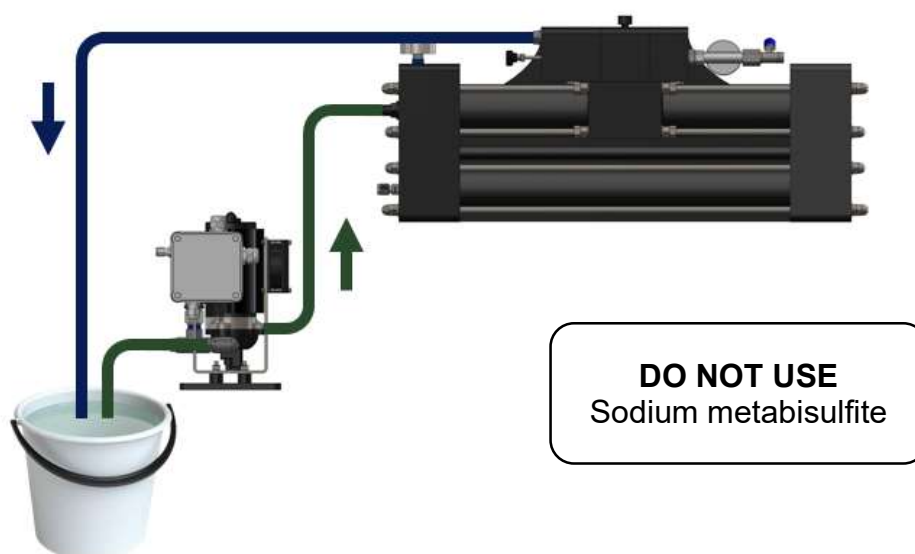
HYDRAULIC SCHEME FOR SHUTDOWN PROCEDURE FIG. 6-1
