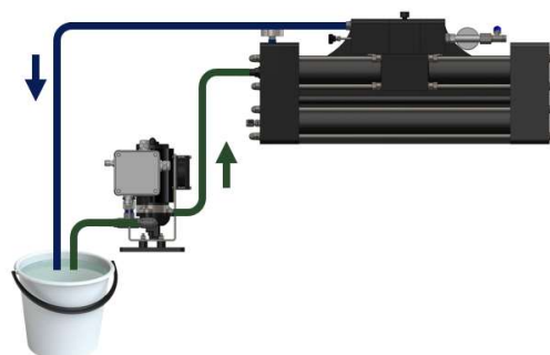
HYDRAULIC SCHEME FOR WINTERIZING PROCEDURE FIG. 6-2
