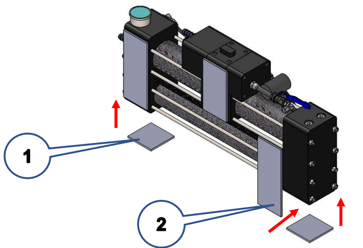
RUBBER STICKER POSITIONS FIG. 4-4
