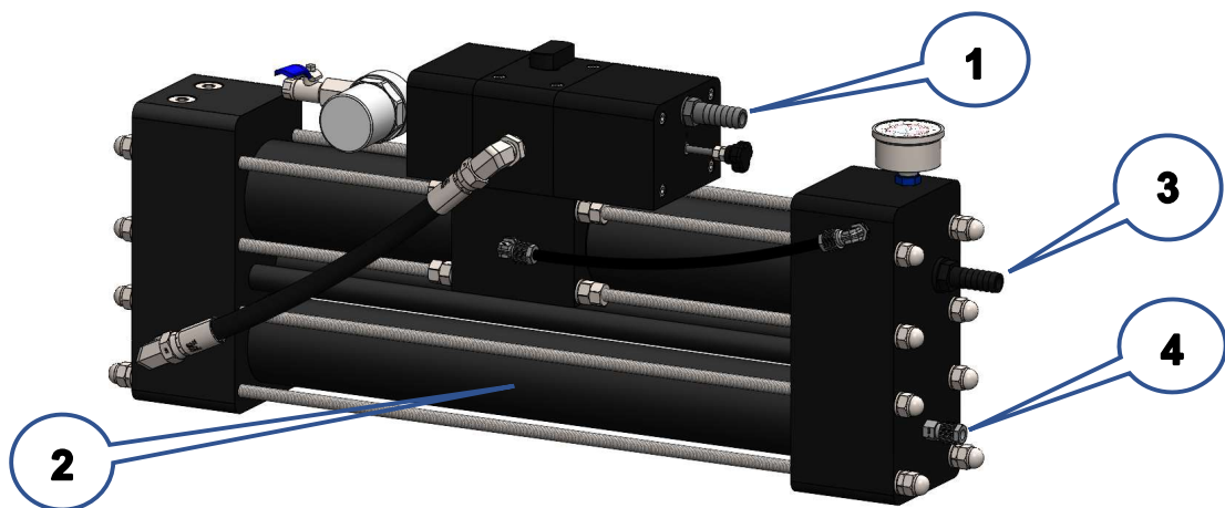
WATERMAKER GROUP (SIDE VIEW W/O COVER) FIG. 3-7
