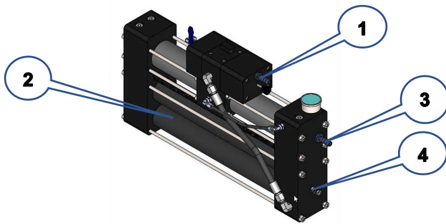
WATERMAKER GROUP (SIDE VIEW W/O COVER) FIG. 3-7
