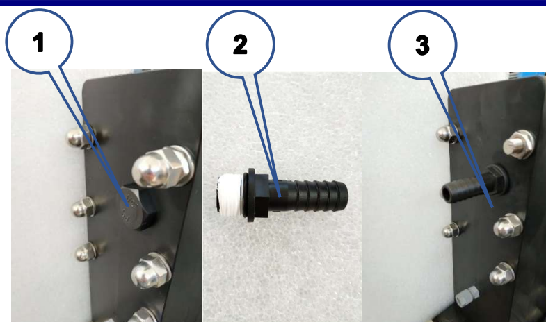
SEAWATER INLET INSTALLATION
