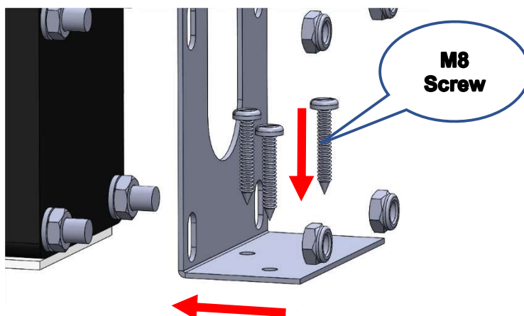
INSTALLATION PROCEDURE FIG. 4-2
